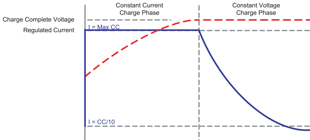
Figure 1: Current vs. Voltage Profile During Charging Phases.
