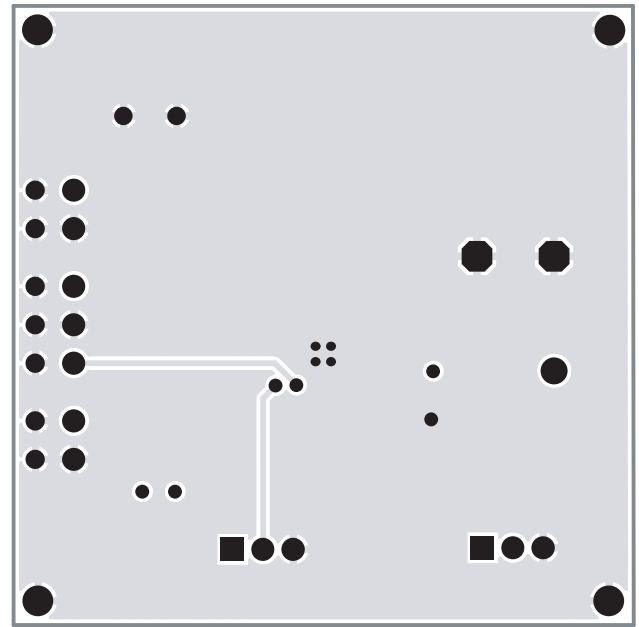
Figure 5: AAT3690 Evaluation Board Bottom Side Layout.
